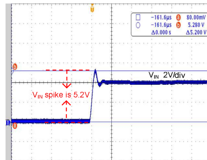
Time (40μs/div) C_{IN}=22\mu F/6.3V/(22\mu F+0.1\Omega)
