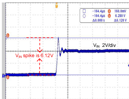
Time (40μs/div) C_{IN}=22\mu F/6.3V
