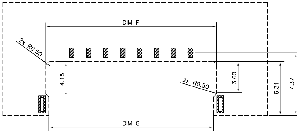
OBVERSE SIDE OF PCB
