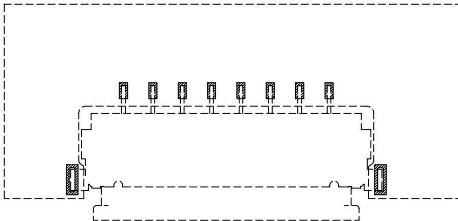
MATING DRAWING
