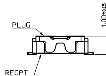
MATING CONDITION
