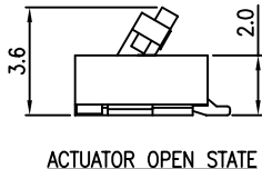
ACTUATOR OPEN STATE
