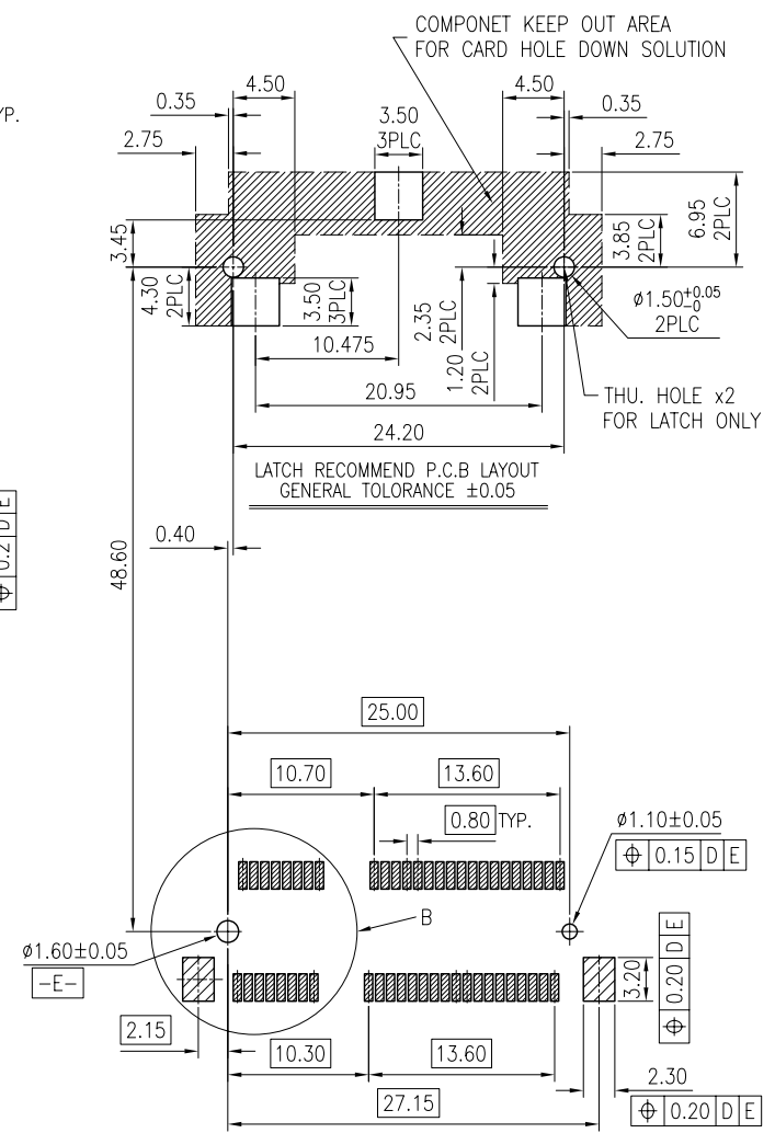
CONNECTOR RECOMMEND P.C.B LAYOUT GENERAL TOLERANCE ±0.05
