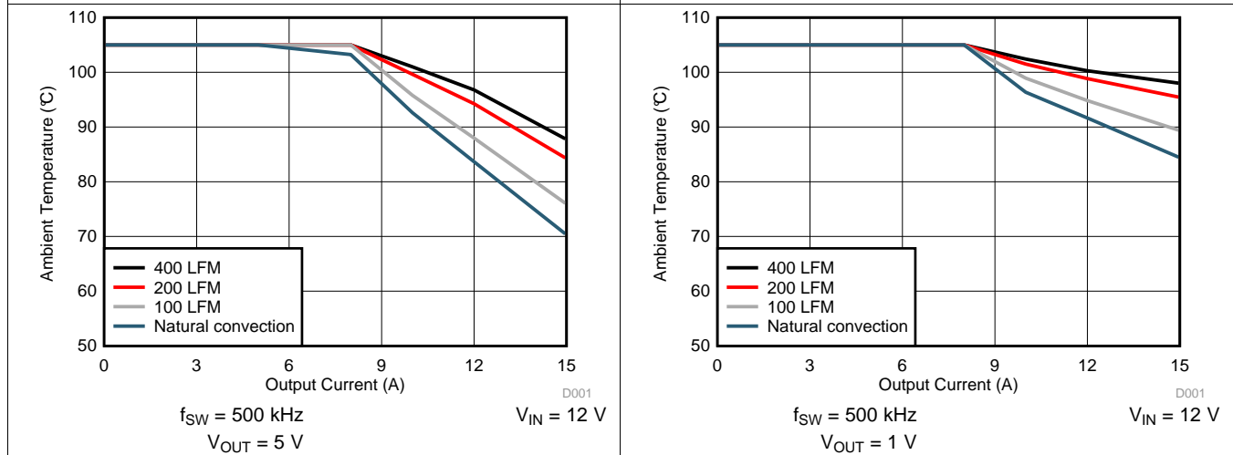
Figure 9. Safe Operating Area
