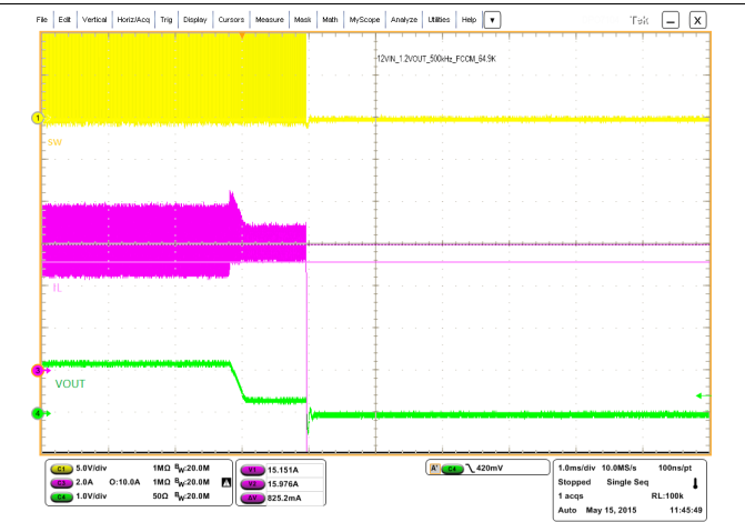
Figure 29. Overcurrent Protection
