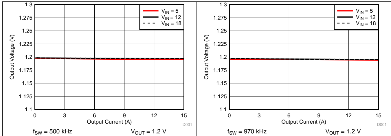
Figure 7. DC Load Regulation
