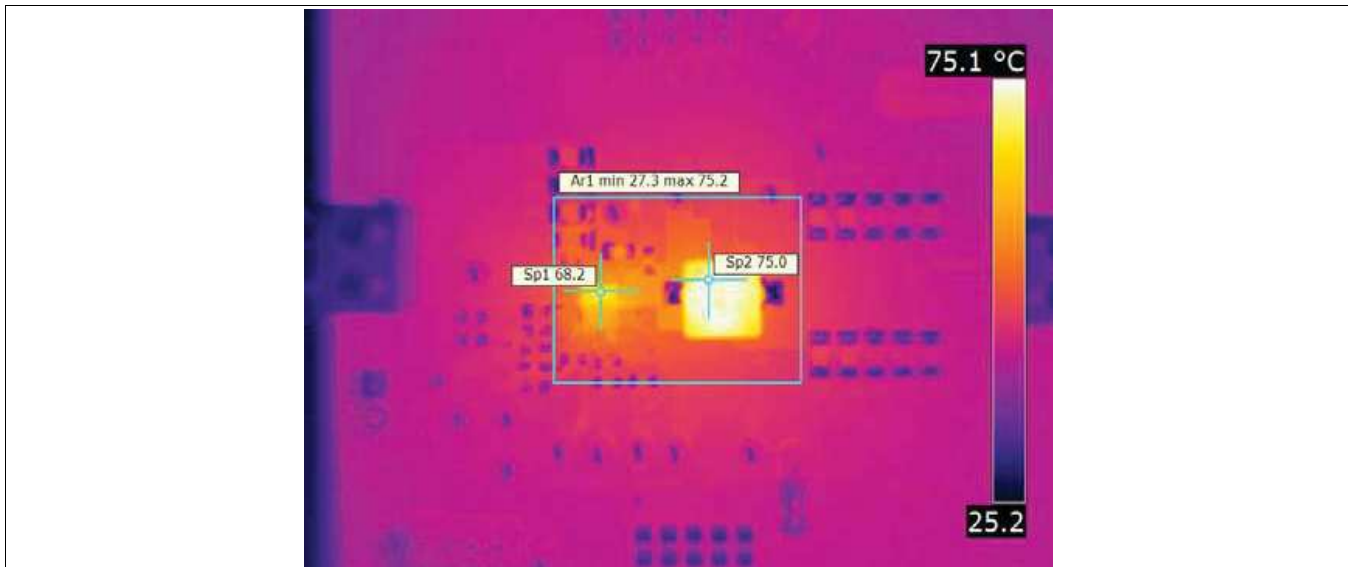
Figure 30. SP1: 68.2°C ( TPS548A20 ), SP2: 75°C (Inductor)
