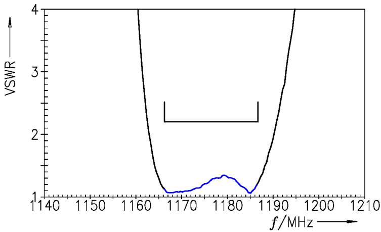
Figure 4: Reflection coefficient at ANT port.
