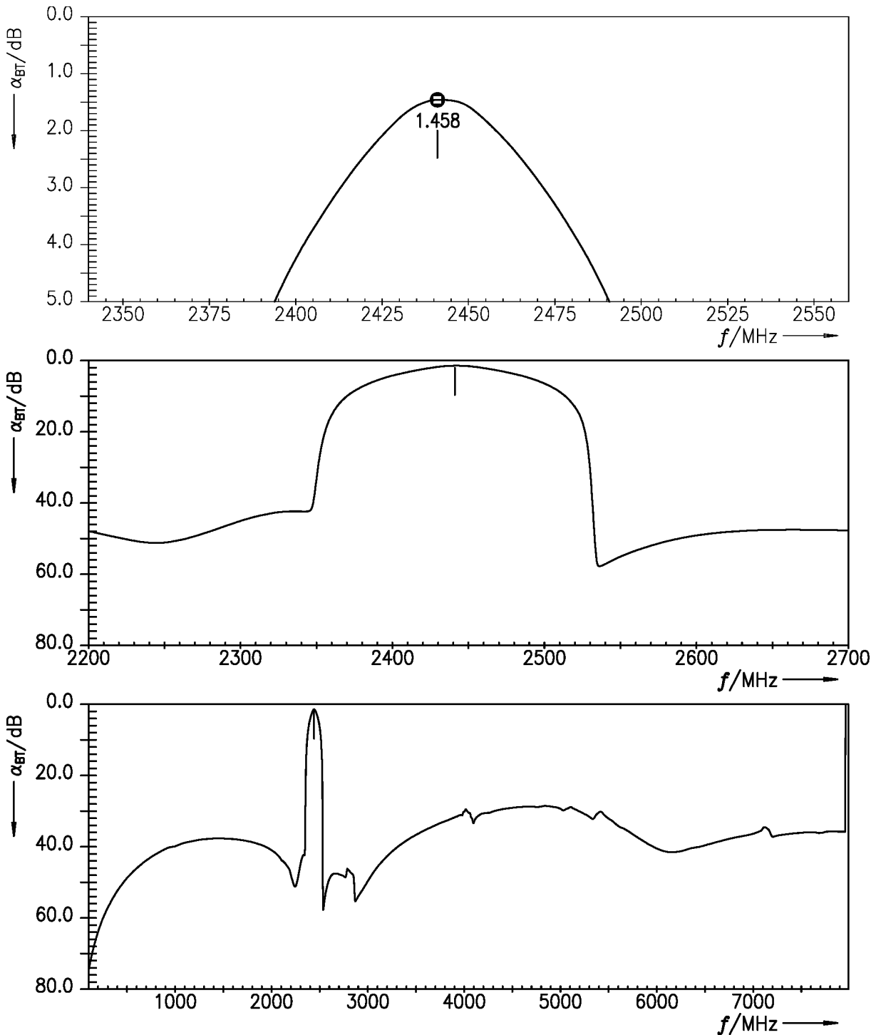
Figure 6: Attenuation (BT) (integration window = 79 MHz).
