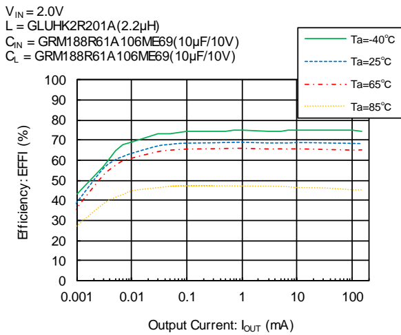
XC9276( V_{OUT}=0.5V )
