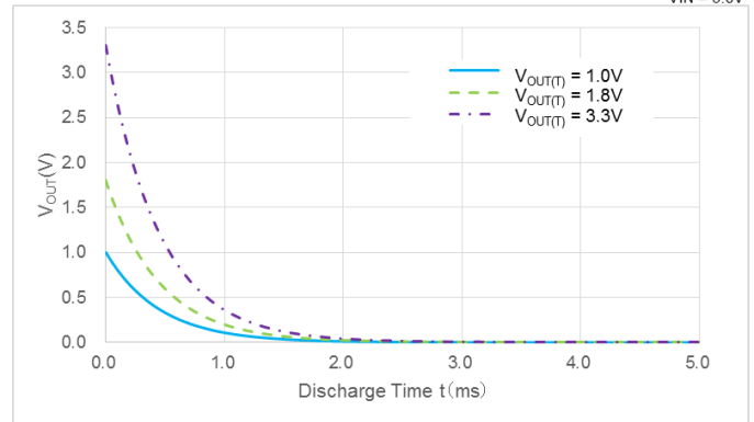
Output Voltage Discharge characteristics
