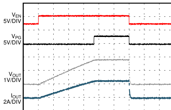
Figure 8-23. Startup without Load
