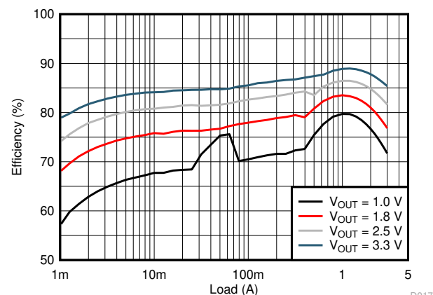
12-V Input Voltage Efficiency
