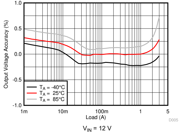
Figure 8-15. Load Regulation
