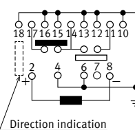
2 coil latching (Reset)
