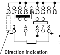
1 coil latching (Reset)
