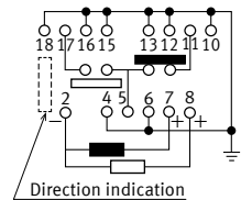
2 coil latching (Reset)
