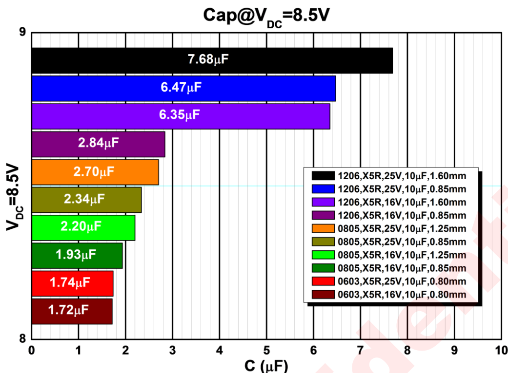
Figure 22 The Space Remaining Value of Different Types of Capacitors at V DC = 8.5V
