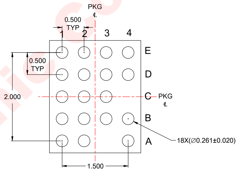
Bottom View
