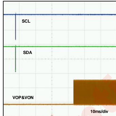
Start-up sequence
