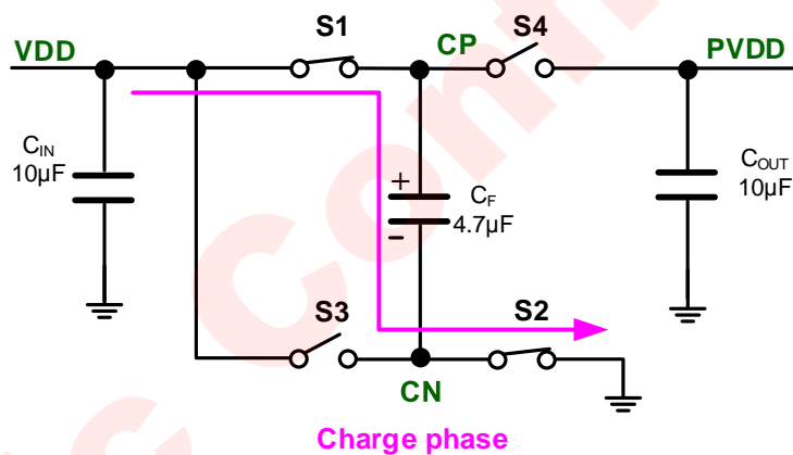
Figure 10 \Phi_1 : Flying Capacitor Charging
