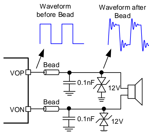
Figure 23 Ferrite Chip Bead and Capacitor
