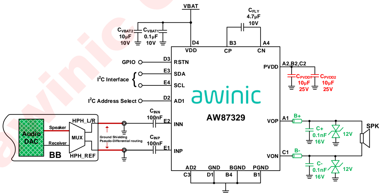
Figure 1 AW87329 Single-ended Input Mode Application Diagram
