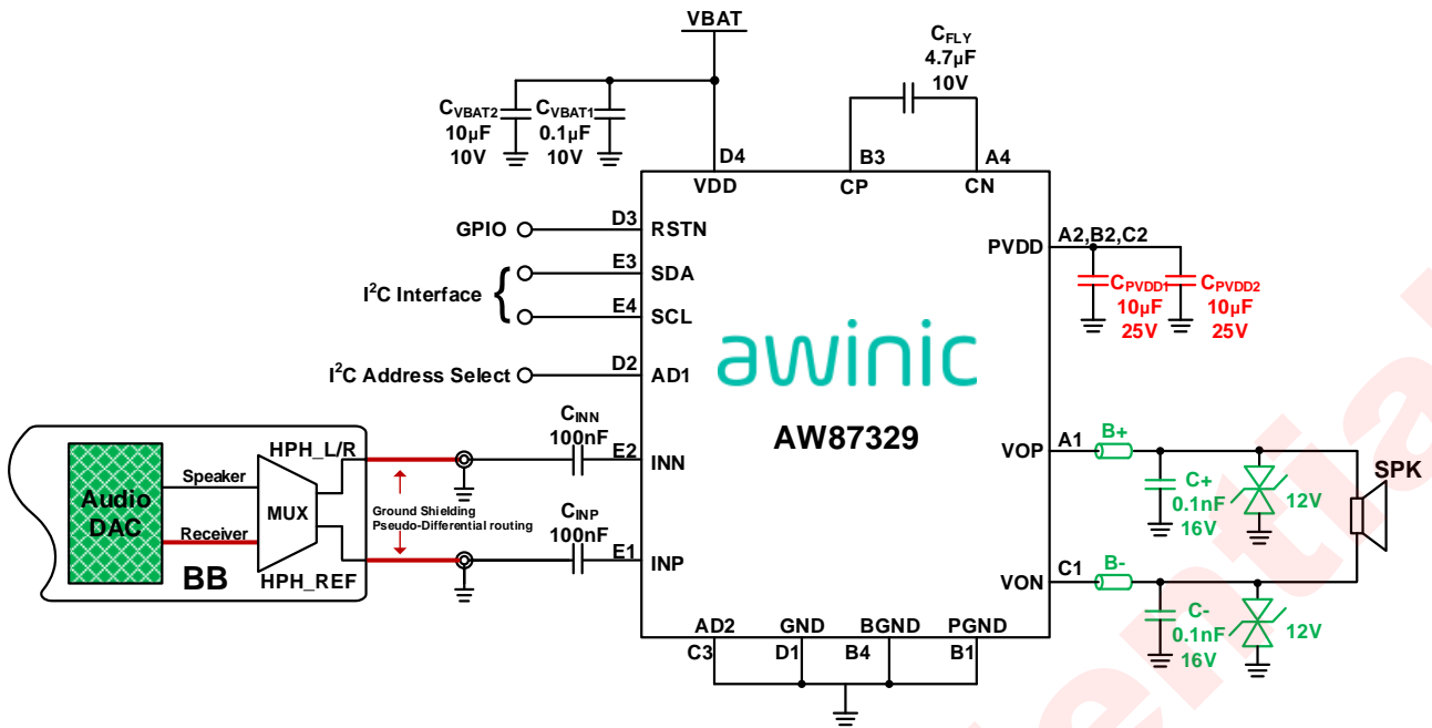
Figure 2 AW87329 Speaker & Receiver 2-in-1 Mode Application Diagram
