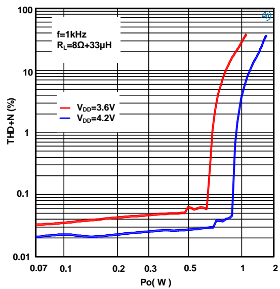
Class D THD+N vs Po
