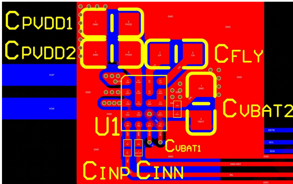
Figure 25 AW87329 Board Layout
