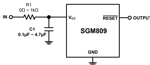
Figure 3. Preventing the High Voltage Spike
