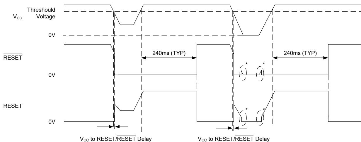
Figure 4. Reset Timing Diagram
