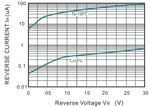
Fig.2 Reverse Characteristics
