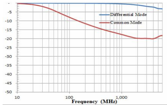
Insertion loss of AMD12012F2SF-900T04
