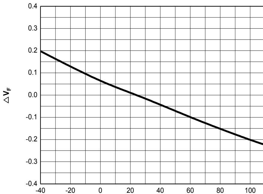
Fig 7. Junction Temperature vs. Forward Voltage Shift, I_F = 30\text{mA}
