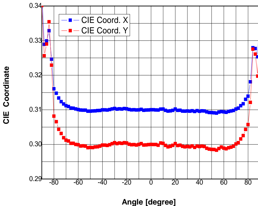
Fig 10. Color. vs. Viewing Angle, T_j = 25^\circ\text{C} , I_F = 30\text{mA}
