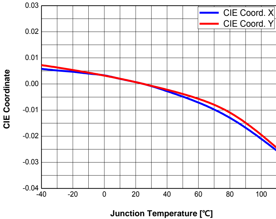
Fig 8. Chromaticity Coordinate vs. Junction Temperature, I_F = 30\text{mA}
