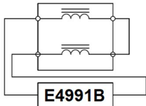
Differential mode
