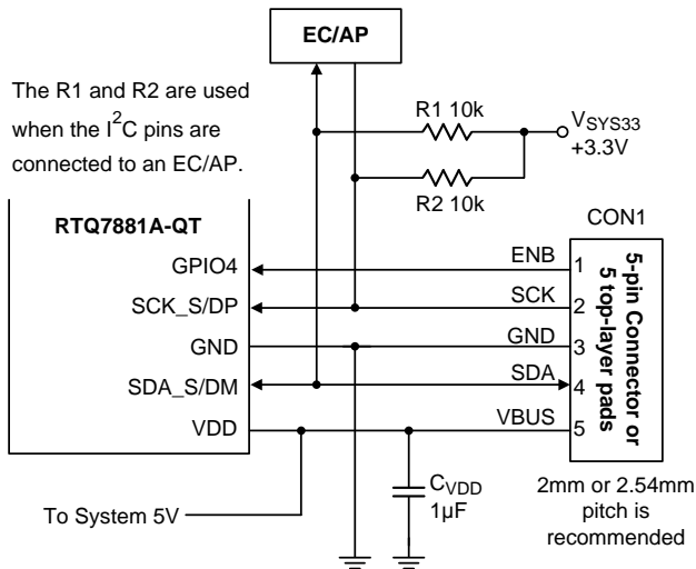
Figure 8. Connections for Manual Firmware Updates
