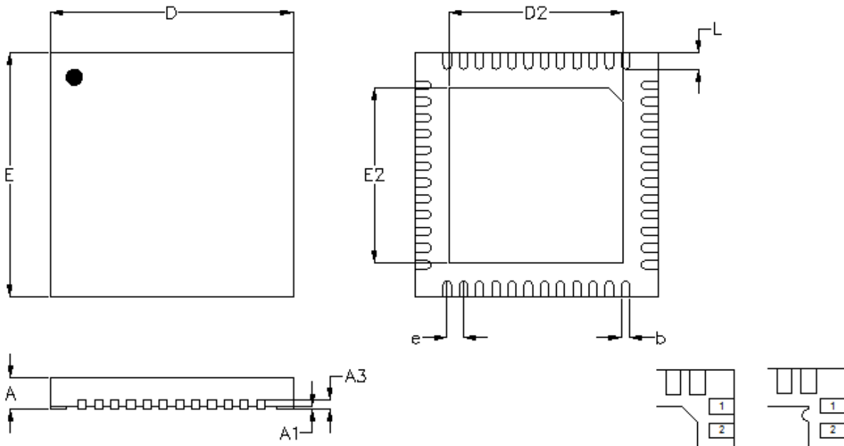
DETAIL A
