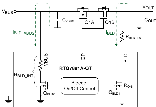
Figure 3. Functional Diagram of the Output Bleeders
