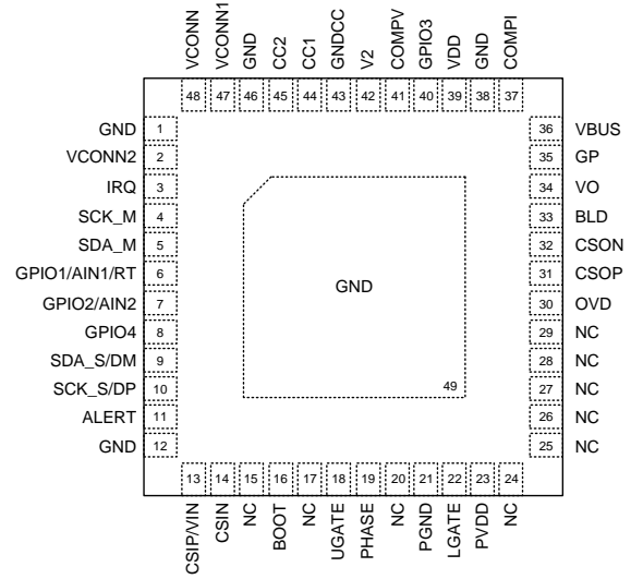
WQFN-48L 6x6
