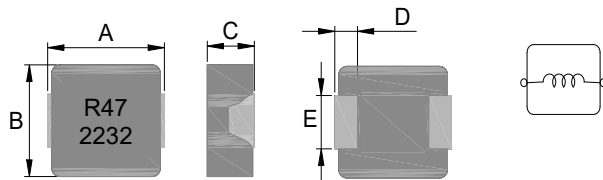
non-leadframe
