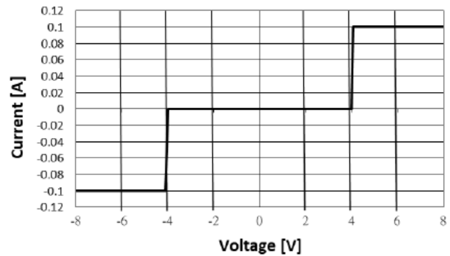
Voltage Sweeping of I/O_1 to I/O_2
