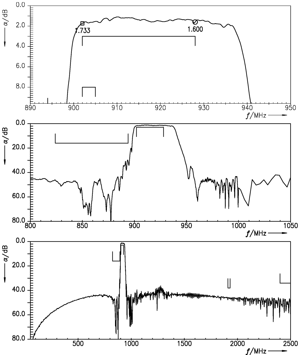
Figure 4: Attenuation Filter1.
