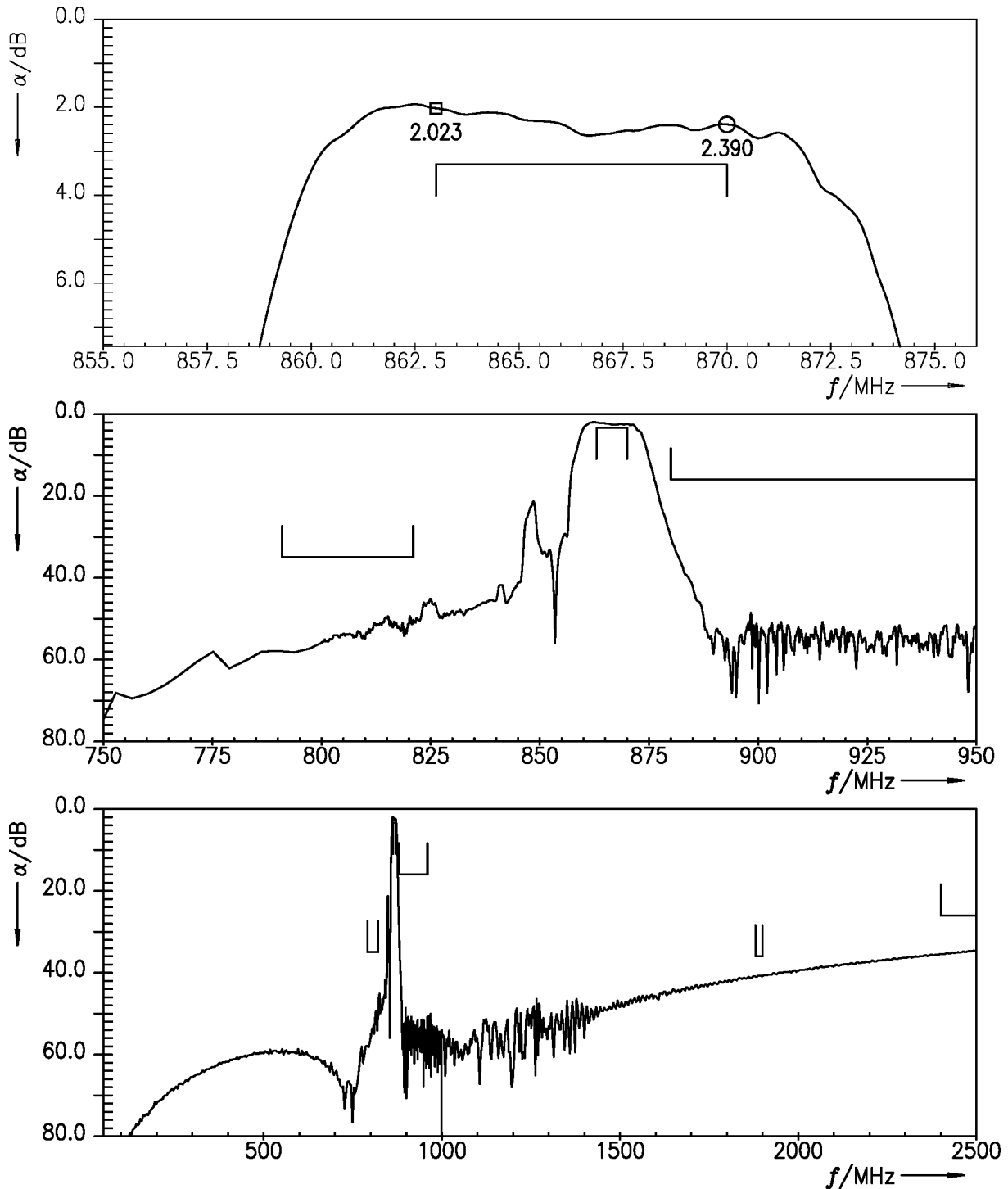
Figure 7: Attenuation Filter2.
