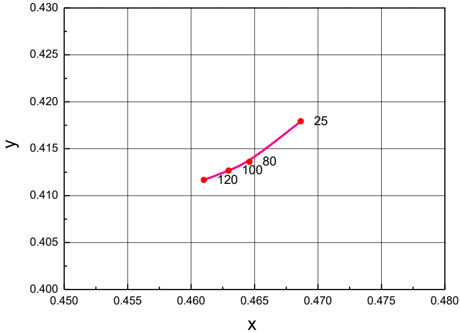
Fig 8. Chromaticity Coordinate vs. Junction Temperature, I_F=100\text{mA} (2600~4200K)
