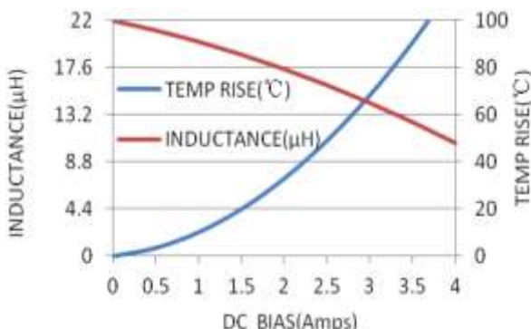
MWSA0624S-220MT
