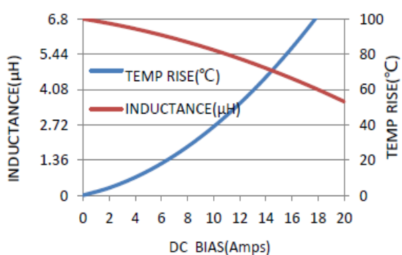
MWSA1204S-150MT
