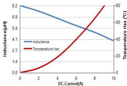
MWSA0605S-8R2MT
