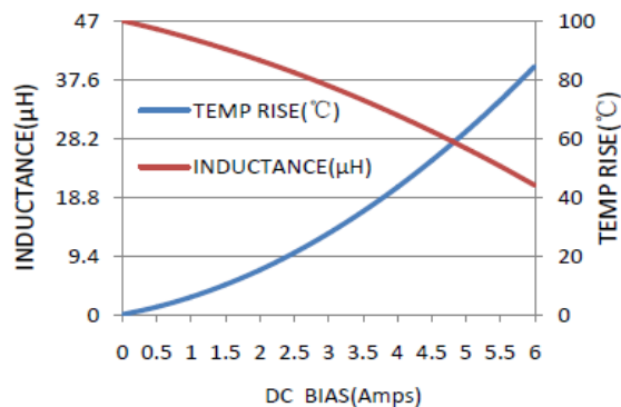
MWSA1004S-470MT
