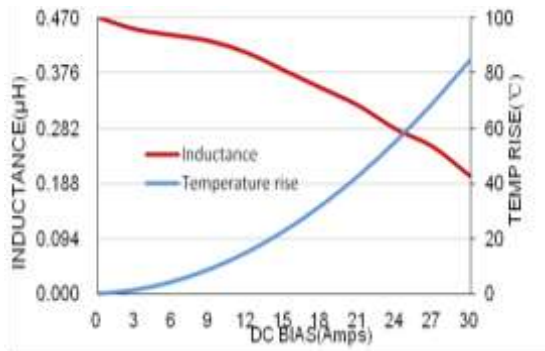
MWSA0603S-R47MT
