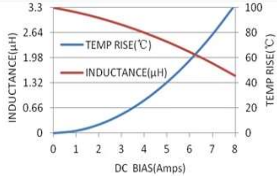
MWSA0518S-6R8MT
