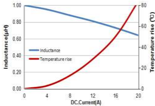
MWSA0605S-1R0MT
