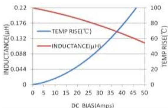
MWSA0603S-R22MT
