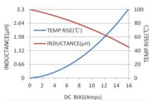
MWSA0603S-3R3MT
