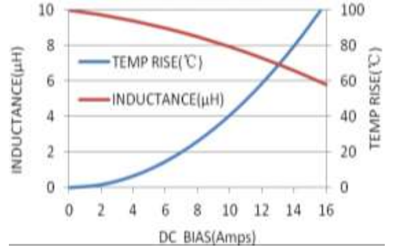
MWSA1205S-220MT
