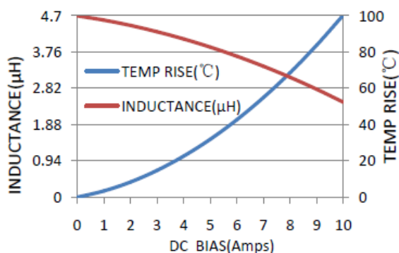
MWSA0624S-100MT
