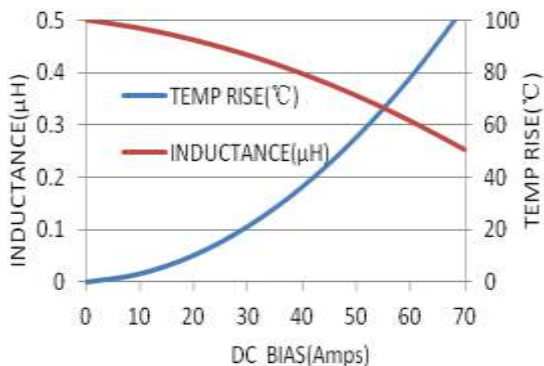
MWSA1205S-R82MT
