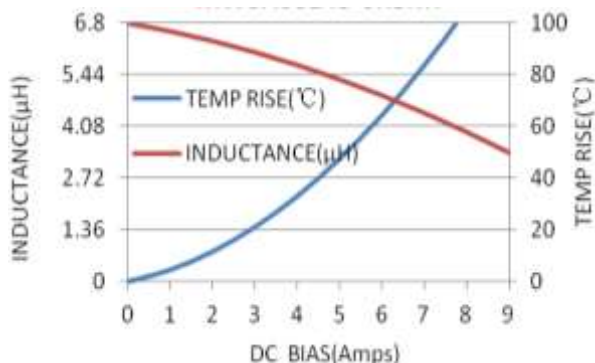
MWSA0624S-150MT
