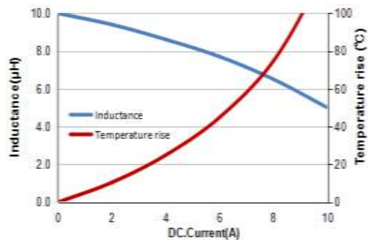
MWSA0605S-100MT
