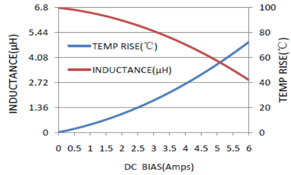
MWSA0503S-6R8MT
