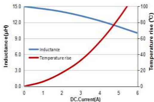
MWSA0605S-150MT
