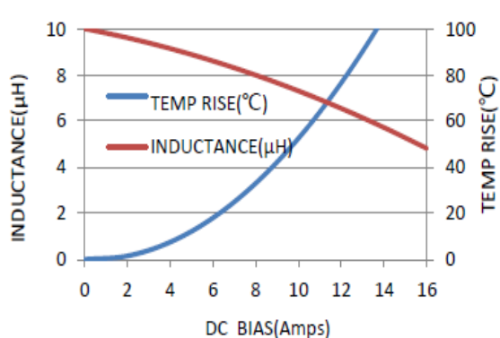
MWSA1204S-100MT
