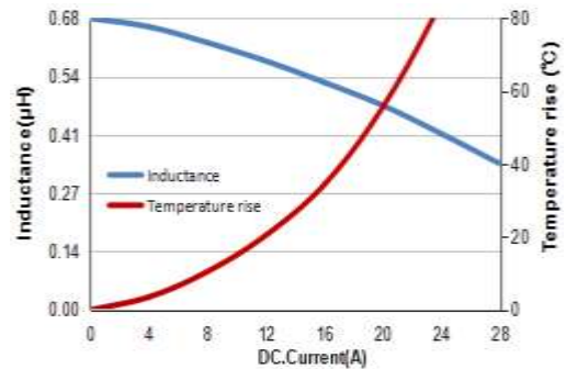
MWSA0605S-R68MT
