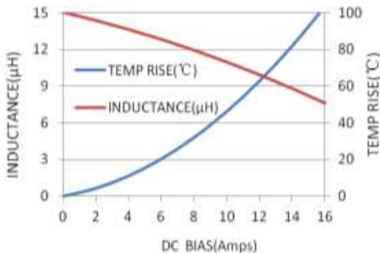
MWSA1205S-150MT
