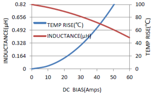
MWSA1204S-R82MT
