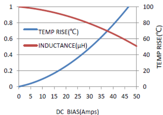
MWSA1204S-2R2MT
