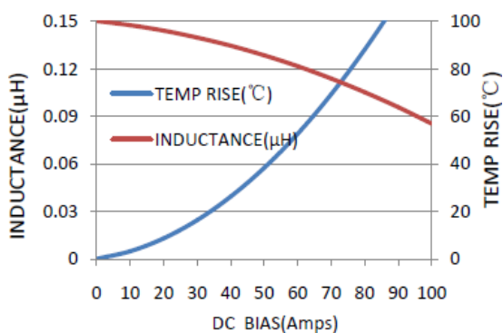
MWSA1004S-R15MT
