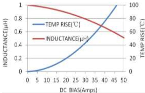
MWSA1205S-1R0MT
