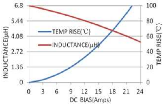
MWSA1205S-150MT
