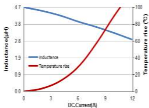
MWSA0605S-4R7MT
