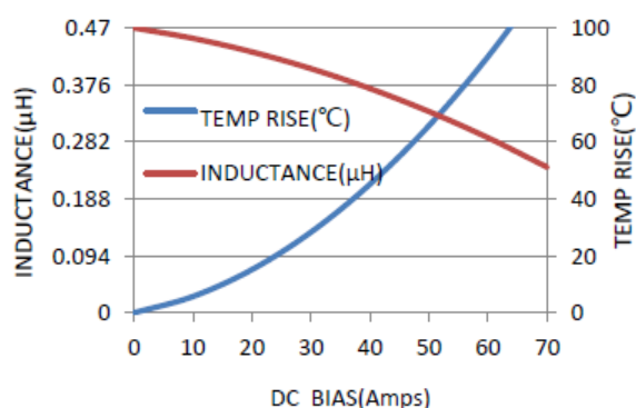
MWSA1204S-R47MT
