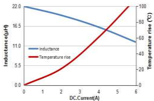
MWSA0605S-220MT
