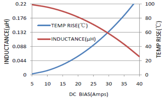
MWSA0618S-R22MT
