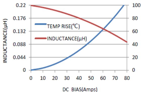
MWSA1204S-R22MT
