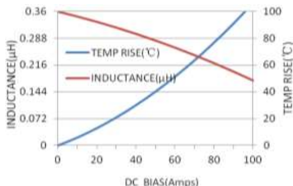
MWSA1205S-R36MT
