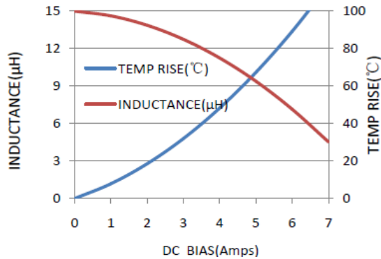
MWSA0603S-150MT
