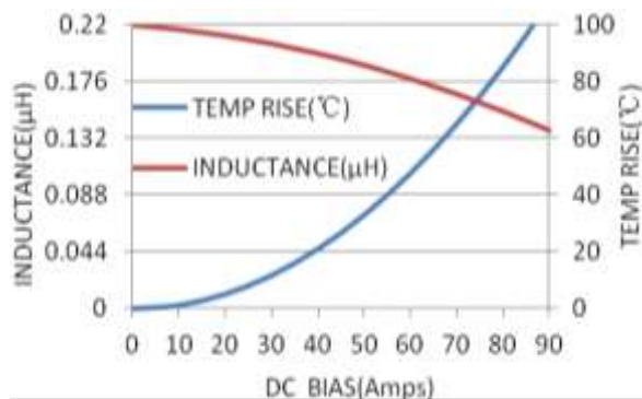
MWSA1205S-R22MT
