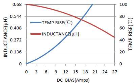
MWSA0618S-R68MT
