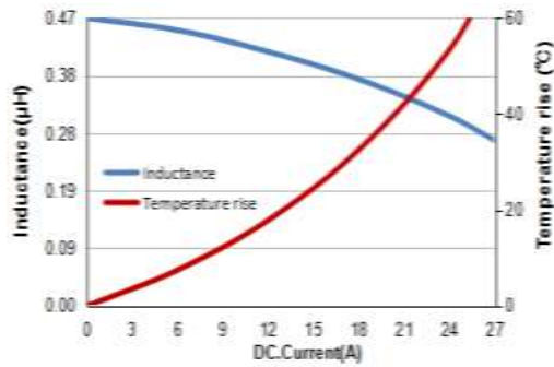
MWSA0605S-R47MT
