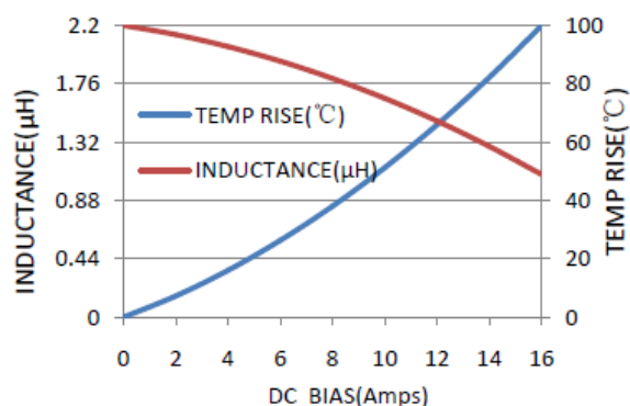
MWSA0624S-2R2MT
