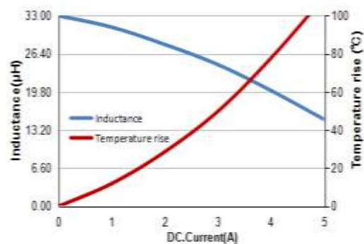
MWSA0605S-330MT
