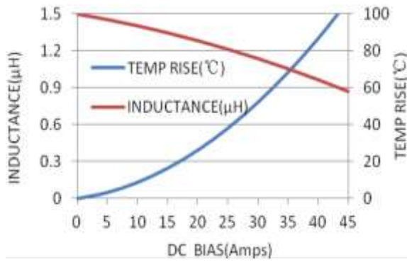
MWSA1205S-3R3MT
