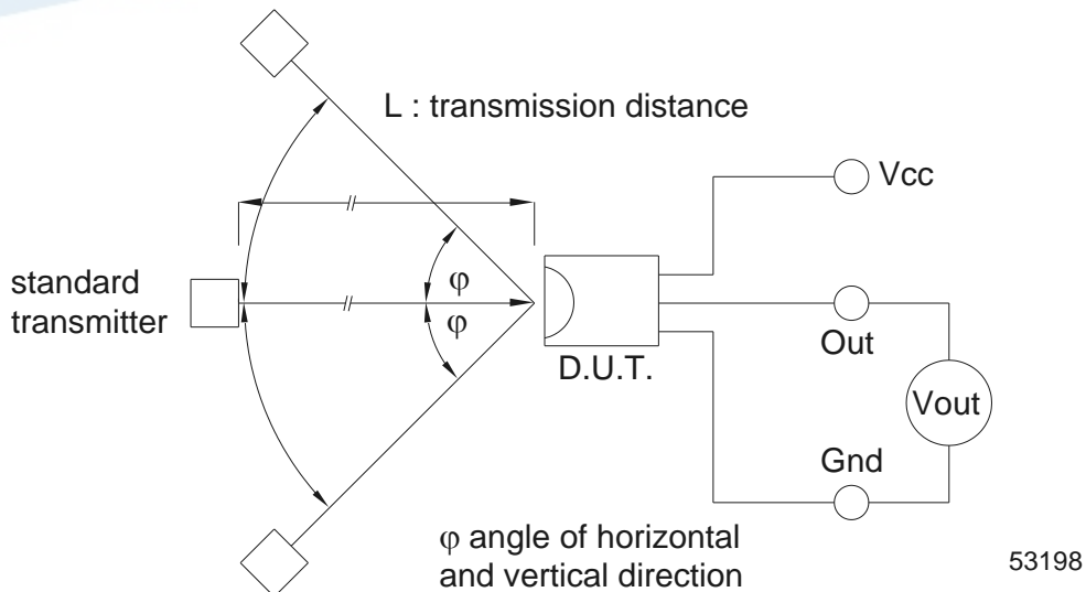
Fig.3 Measuring System
