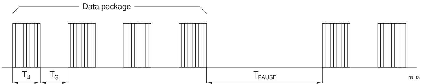
Fig.14: general IR data structure
