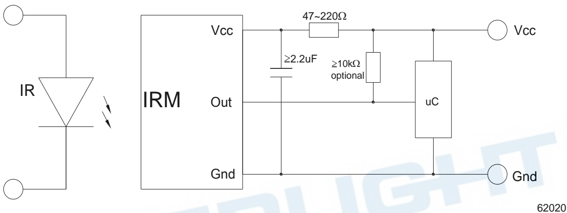
Fig.13: application circuit
