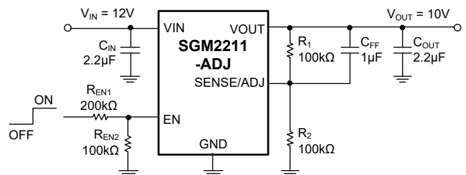
Figure 7. Adjustable Output Voltage Application
