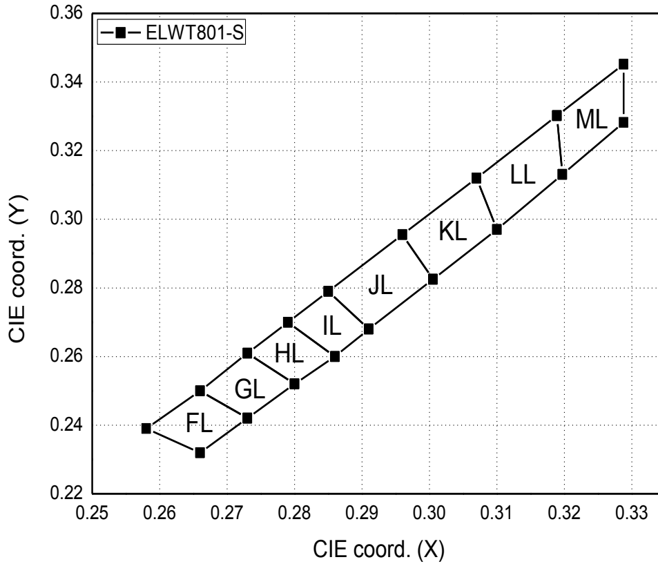
CIE Chromaticity Diagram, I_F = 20\text{mA} , T_j = 25^\circ\text{C}
