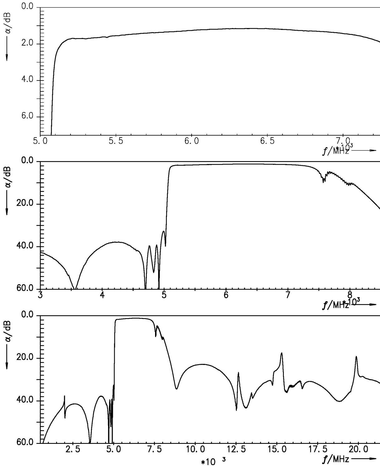
Figure 4: Attenuation.
