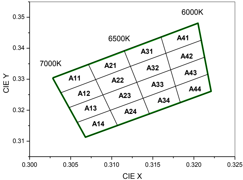
CIE Chromaticity Diagram (Cool white), T_j=25^\circ\text{C} , I_f=65\text{mA}
