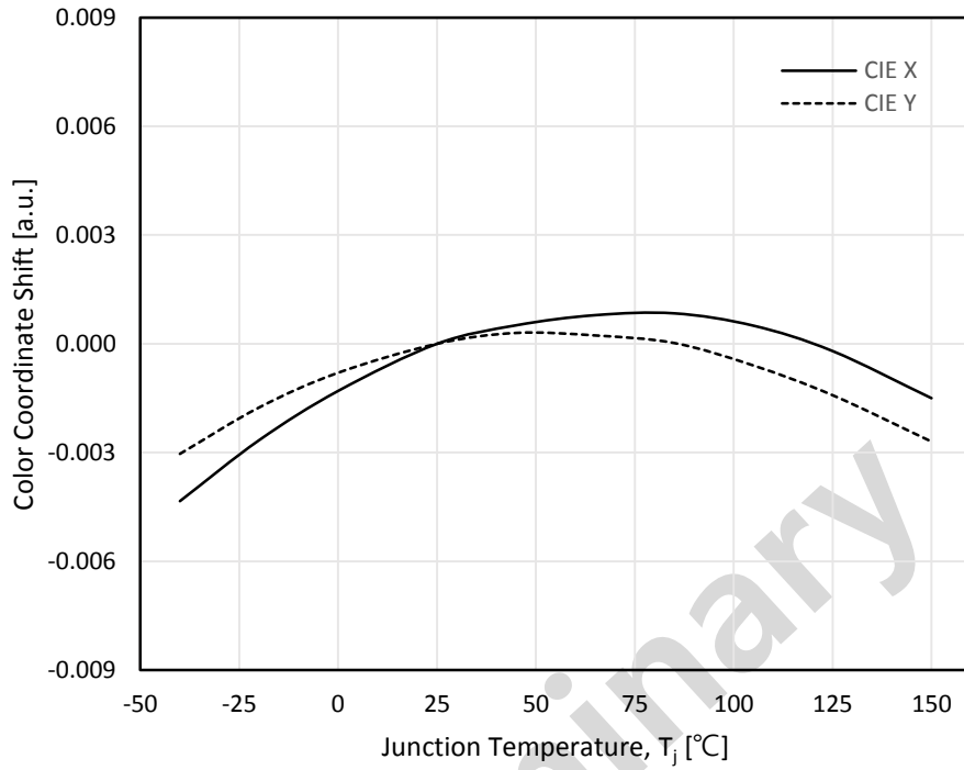
Fig 8. Junction Temperature vs. Color Coordinate Shift, I_F= 1.0A
