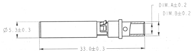
SOCKET (FEMALE)
