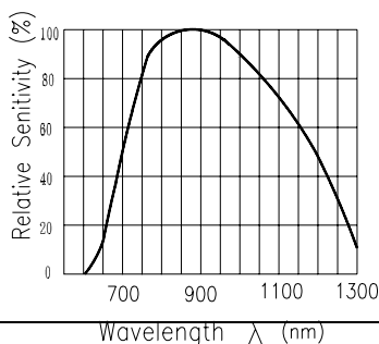
Fig.5 Spectral Sensitivity
