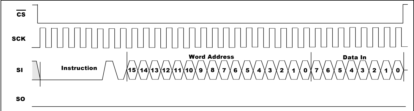
Figure 5-7. WRITE Timing
