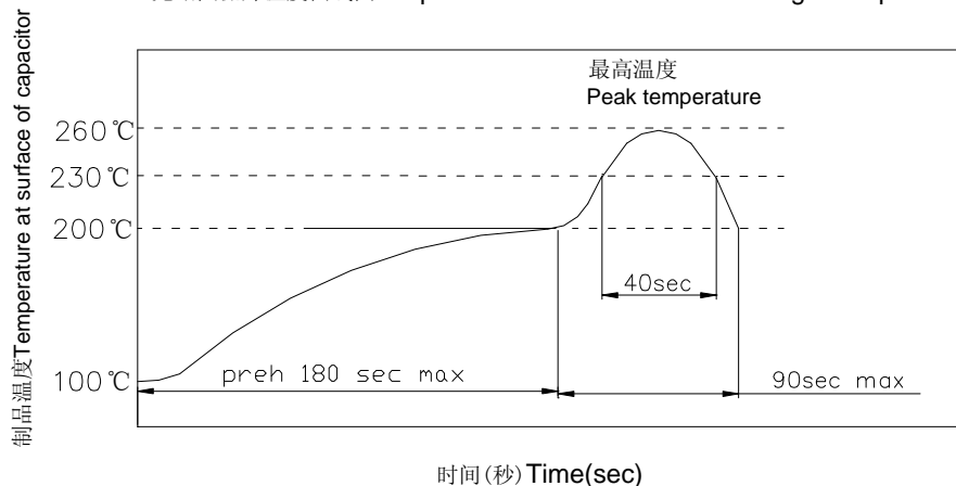
无铅回流焊温度曲线图 Graph for Lead-free reflow sold cringe temperature
