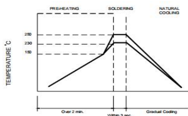
Figure 2. Wave Soldering
