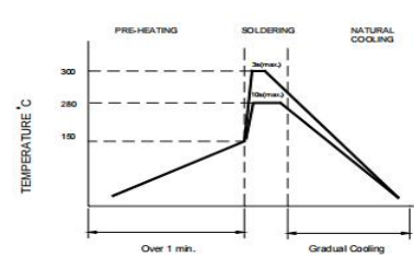
Figure 3. Hand Soldering
