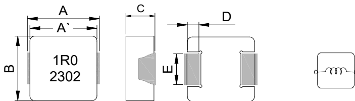
non-leadframe
