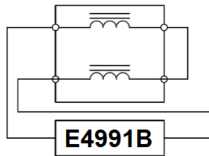
Differential mode
