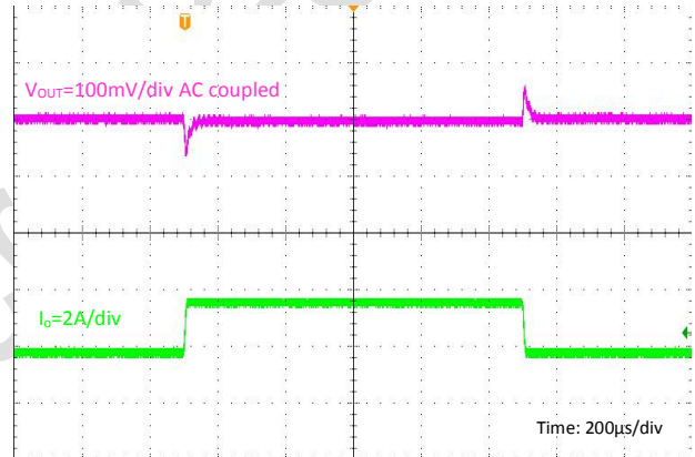
Load Transient
