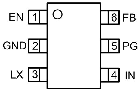
SOT23-6 (Top View)
