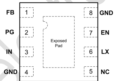
DFN2x2-8 (Top View)
