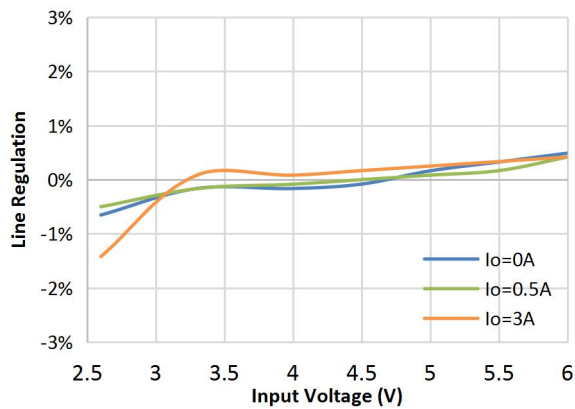
Line Regulation at V_{OUT}=1.2V
