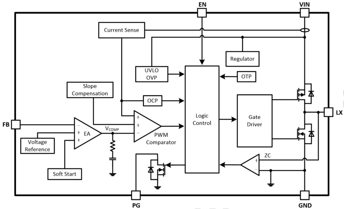
Figure 2. TMI3113H2 and TMI3113H2D Block Diagram
