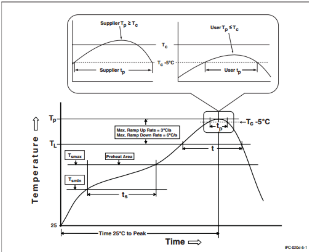
Figure 5-1 Classification Profile
