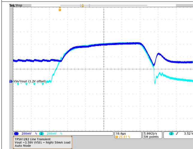
Figure 43. TPS61281A Forced Pass-Through to Boost Mode Transition
