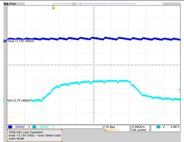
Figure 62. TPS61282A Line Transient
