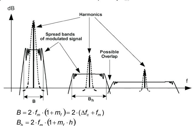
Figure 16. Spread Bands of Harmonics in Modulated Square Signals (1)
