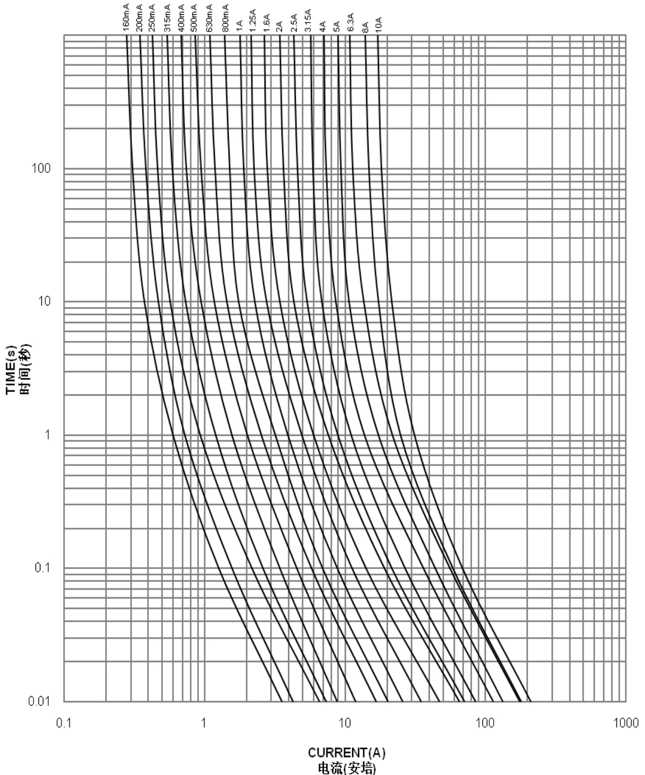
DETRoHS 平均I-T曲线图(仅供参考) DETRoHS AVERAGE I-T CHARACTERISTICS CURVE(FOR REFERENCE ONLY)
