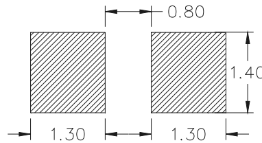
Recommended Soldering Pattern for Top Looker
