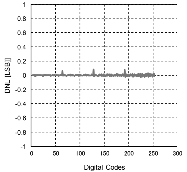
Fig.46 VCOM DNL
