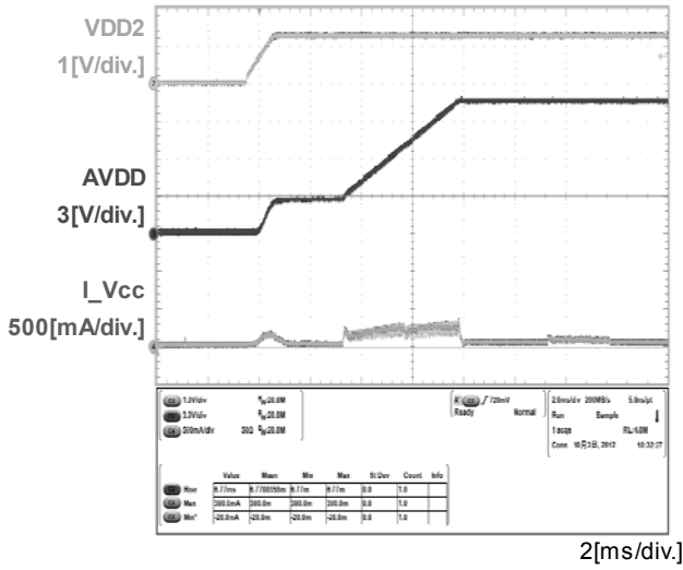
Fig.20 AVDD Start-up Sequence
