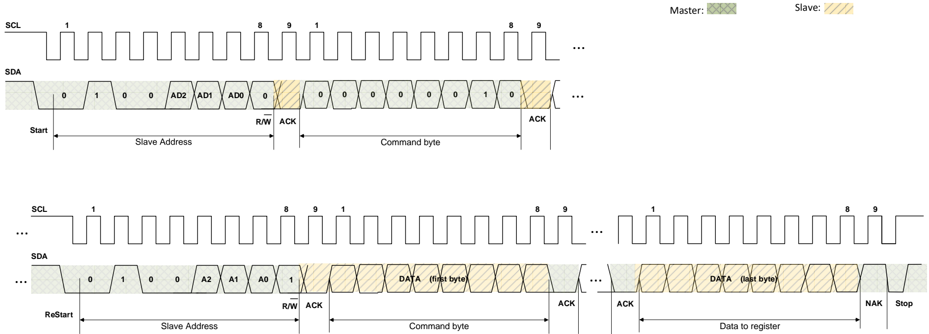
Figure 9. Read from register
