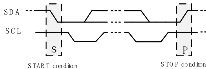
Figure 12. Definition of START and STOP conditions
