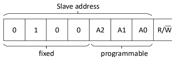
Figure 5. CA9535 device address
