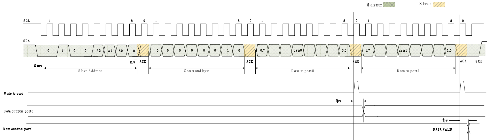
Figure 7. Write to Output port registers
