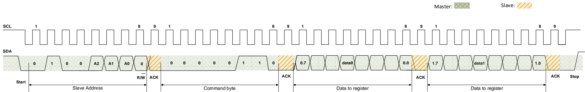
Figure 8. Write to Configuration registers
