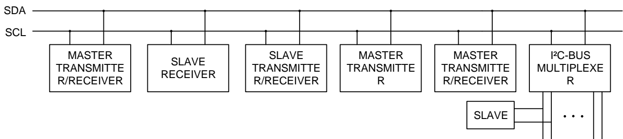
Figure 13. System configuration
