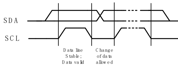
Figure 11. Bit transfer
