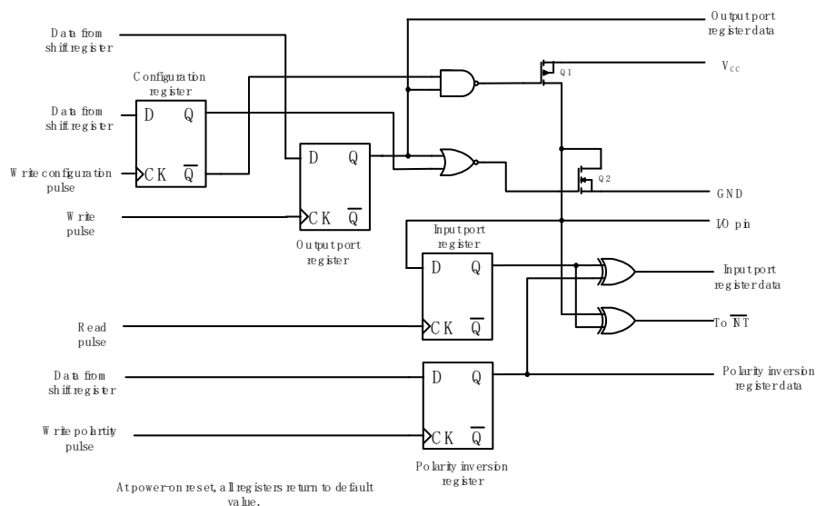
Figure 6. Simplified schematic of I/Os
