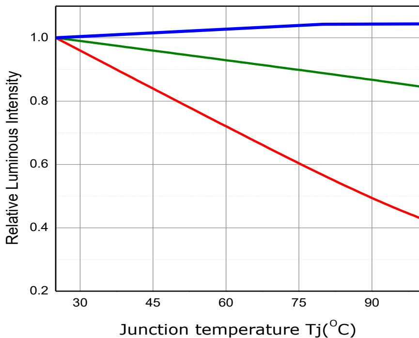
Fig 5. Junction Temperature vs. Relative Luminous Intensity, I_F=20\text{mA}
