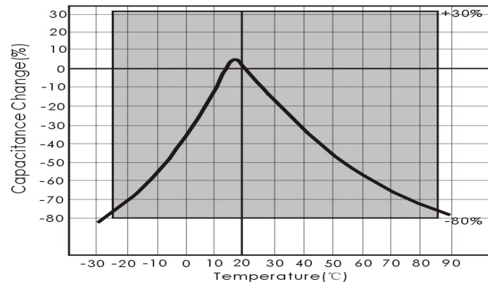
Char:F (Y5V)
