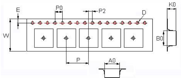
Tape Dimensions
