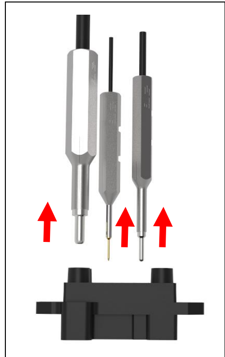
Step4: Pull and remove the contact out of insert
