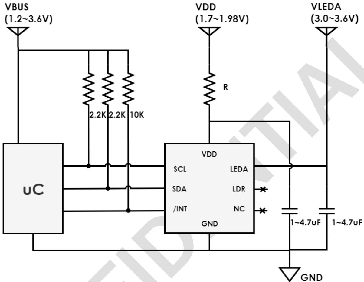
W2301 Typical Application Circuit with Independent VDD and VLED Supply Voltage
