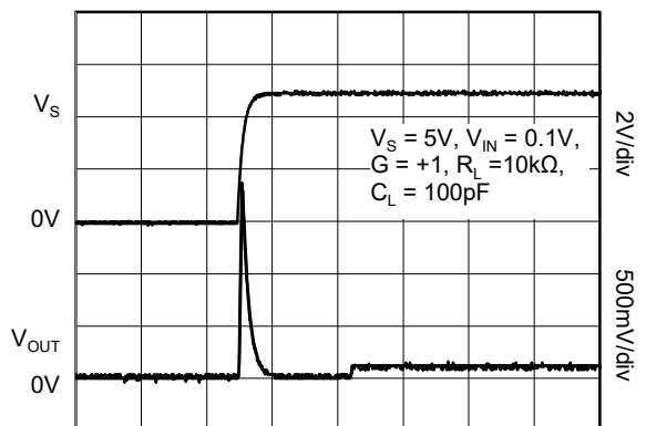
Time (20 \mu\text{s}/\text{div} )
