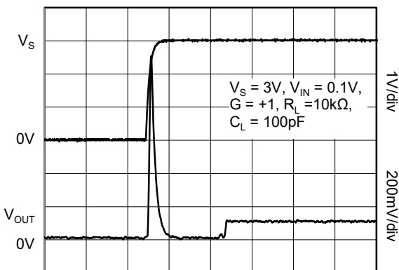
Time (20 \mu\text{s}/\text{div} )
