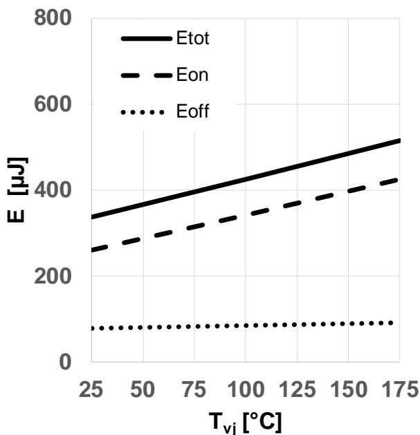
Figure 15 Typical switching energy losses as a function of junction temperature (E = f(T_{vj}), V_{DD} = 800\text{V}, V_{GS} = 0\text{V}/18\text{V}, R_{G,ext} = 2\Omega, I_D = 25\text{A}, \text{ind. load, test circuit in Fig. E, diode: body diode at } V_{GS} = 0\text{V})
